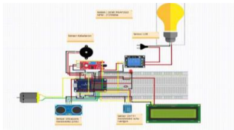
Gambar 1.1 Rangkaian Smart Home
